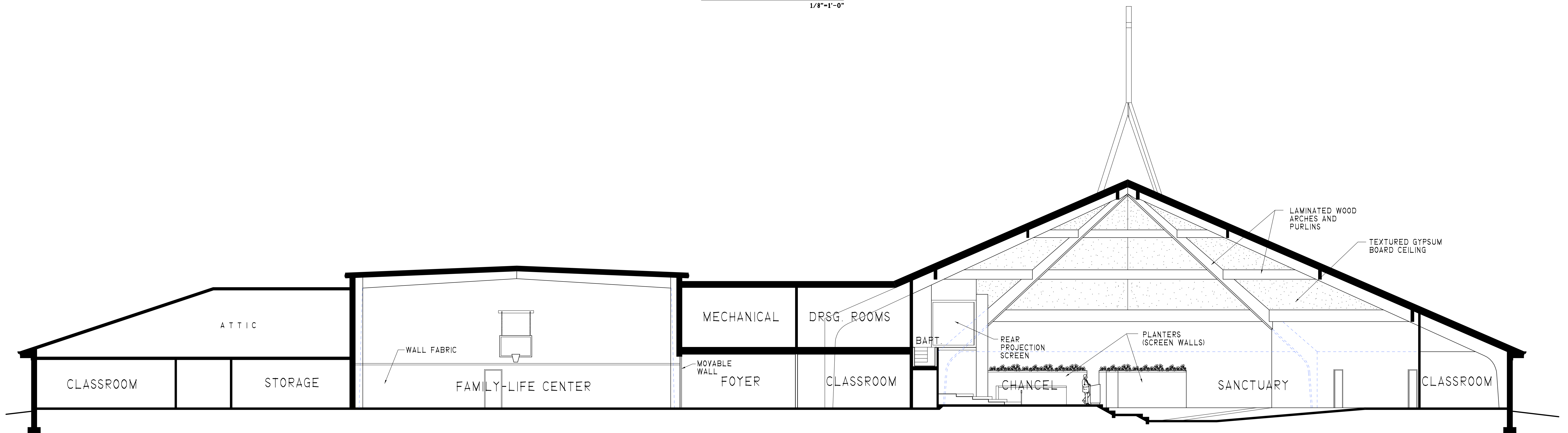
CROSS SECTION 1/8"=1'-0"
